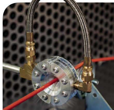
A 3/8" Super Air Wipe uniformly dries a hose as it exits a cooling bath.
